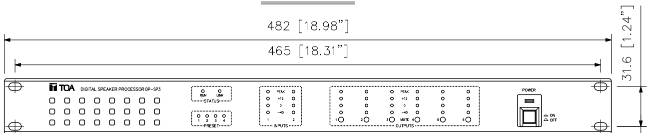
Front View
